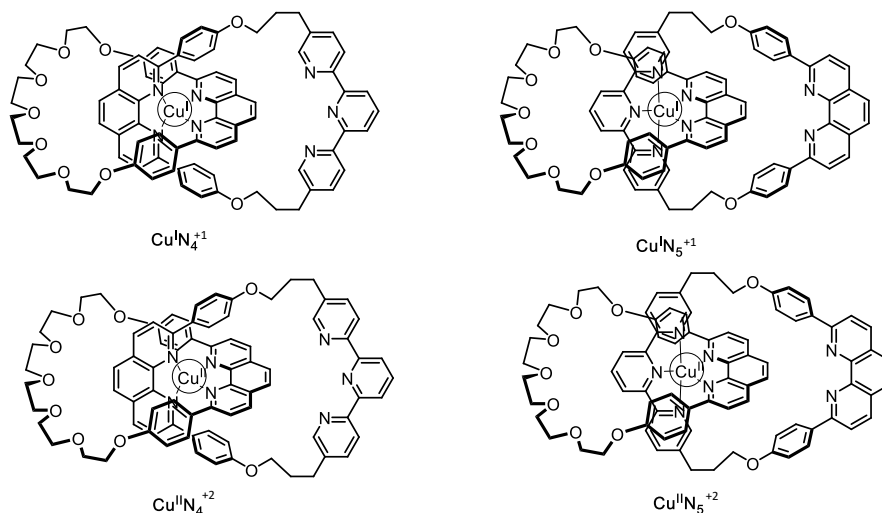
Fig. 2 – [2]catenane L states
