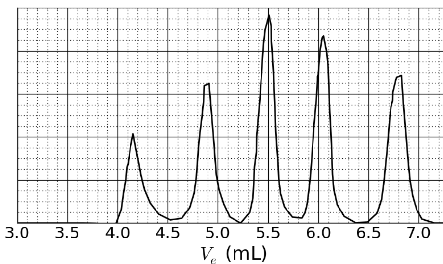
Fig. 3 – SEC chromatogram of the mixture of standards.
